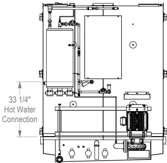
Rear View
